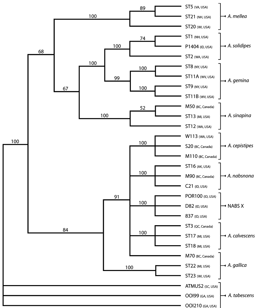
Fig. 1 A 50% majority-rule consensus tree of ten North American Armillaria species based on 24,001 trees from Bayesian inference analysis of the translation elongation factor 1- \alpha gene. Numbers between clades indicate posterior probability. Sequence alignments can be found in TreeBASE (S11603)
